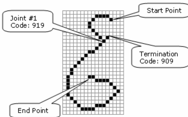
Figure 3: The stroke sequence string for the character Am is 34445567777919190991955545555565666667777000100111133344434.
